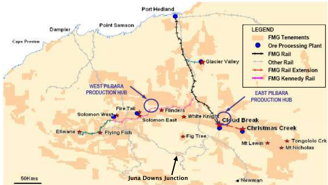
Figure 5-1 Current and proposed railways close to the Hamersley Railway
